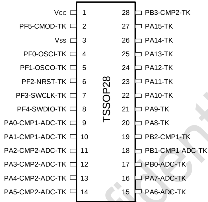
图 3-1 TSSOP28 Pinout1 PY32T020G1xP7-B (Top view)
