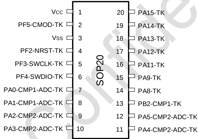
图 3-8 SOP20 Pinout1 PY32T020F1xS7-B (Top view)
