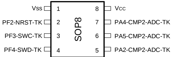
图 3-12 SOP8 Pinout1 PY32T020L1xS7-B (Top view)
