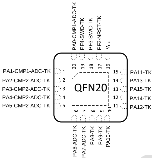
图 3-10 QFN20 Pinout4 PY32T020F4xU7-B (Top view)
