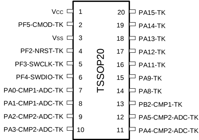
图 3-7 TSSOP20 Pinout1 PY32T020F1xP7-B (Top view)
