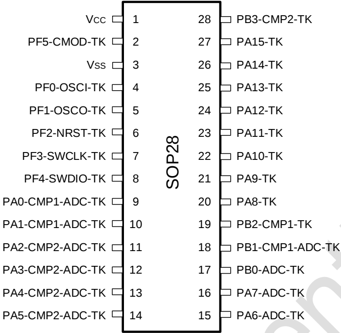
图 3-3 SOP28 Pinout1 PY32T020G1xS7-B (Top view)
