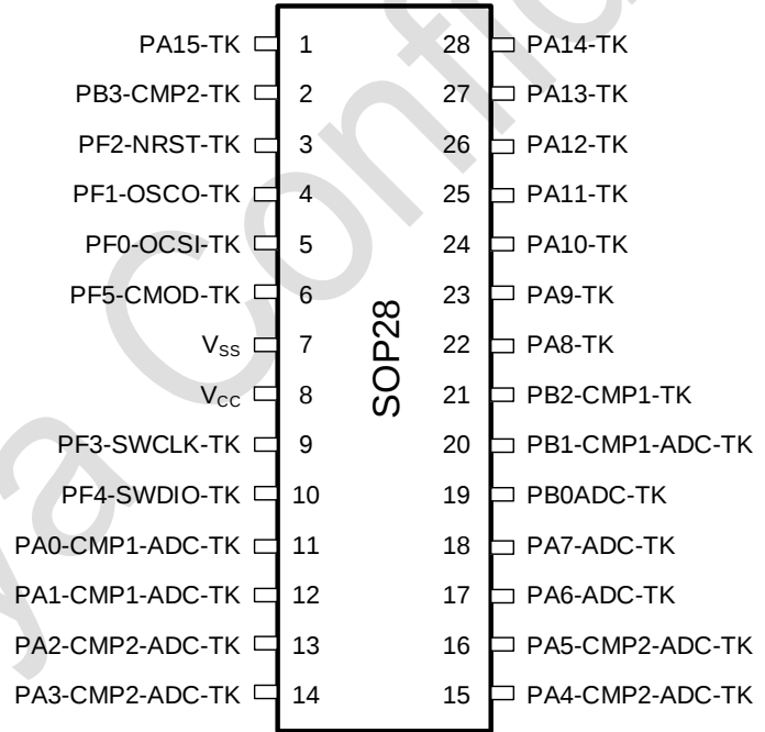
图 3-4 SOP28 Pinout2 PY32T020G2xS7-B (Top view)
